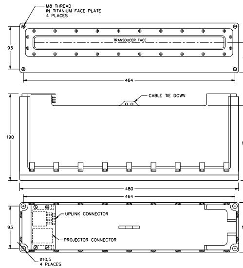
Sonic 2026 Receiver
